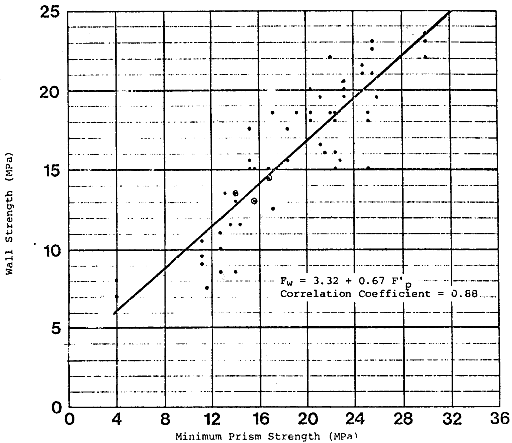
Figure 5. Wall strength ( F_w ) V. Minimum ultimate prism strength ( F'_m )
